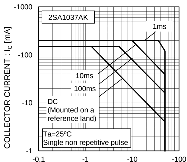
Fig.15 Safe Operating Area
